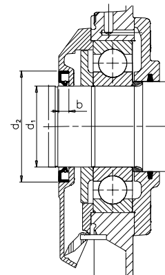
Radial seal
