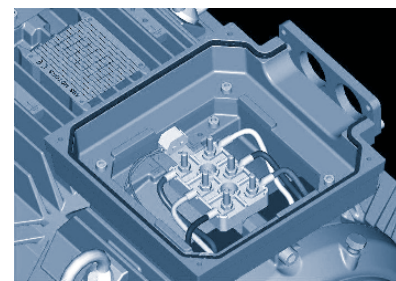
Terminal box for motor sizes 160 to 250
