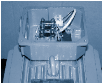
Terminal box for motor sizes 71 to 132
