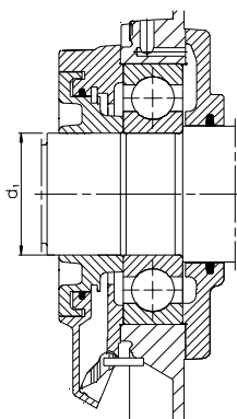
Labyrinth seal
